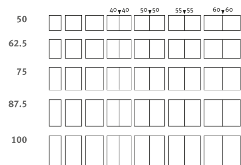
Standard single door with doorstop on left.
